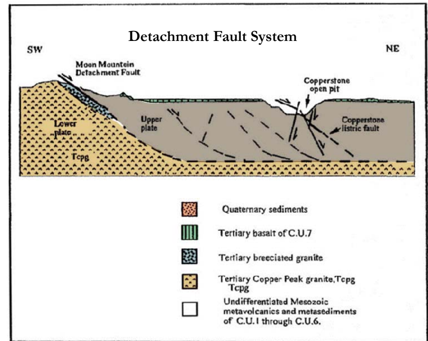
Source: Michael R. Pawlowski, P.Geo, January 2005 Schematic cross-section of the Moon Mountain Detachment Fault and the Copperstone Listric Fault, Solid heavy lines are observed faults; broken line and projected faults.
