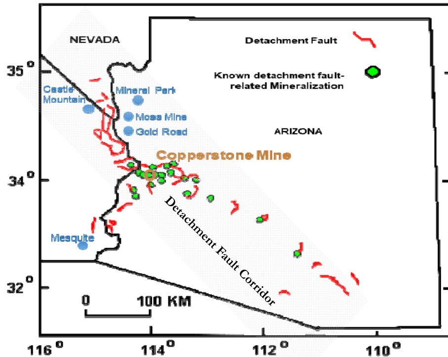
Source: USGS Keith R Long Preliminary Descriptive Deposit Model for Detachment Fault Related Model
